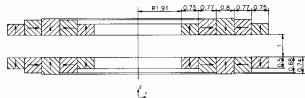
Fig. 3 An design example of optimized Halbach type magnetic bearing
