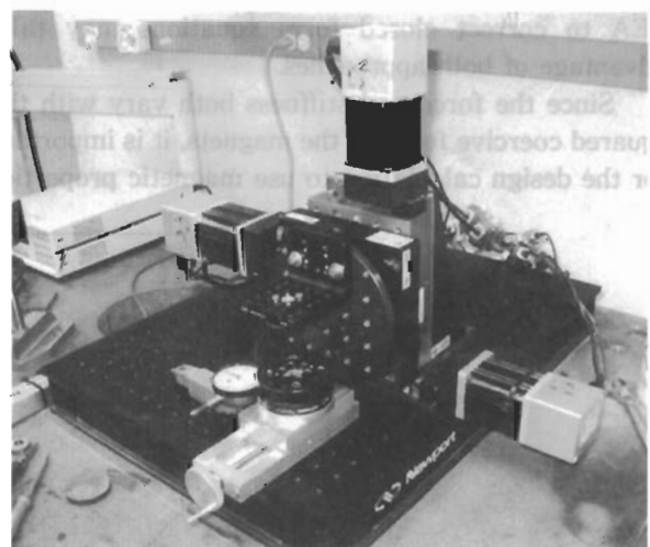
Fig. 5 The stiffness test fixture, showing the positioning stage and the force cell
