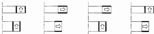
Fig. 1 Basic combinations of magnet rings in a bearing unit and their equivalent current sheets (dashed line is axis of symmetry; only half section is shown)
