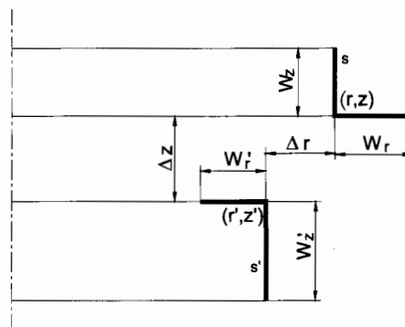
Fig. 2 A pair of L-shaped current sheets for analysis
