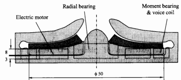
Fig. 4 Schematic cross sectional view of the HeartQuest™ VAD showing the magnetic bearing configuration
